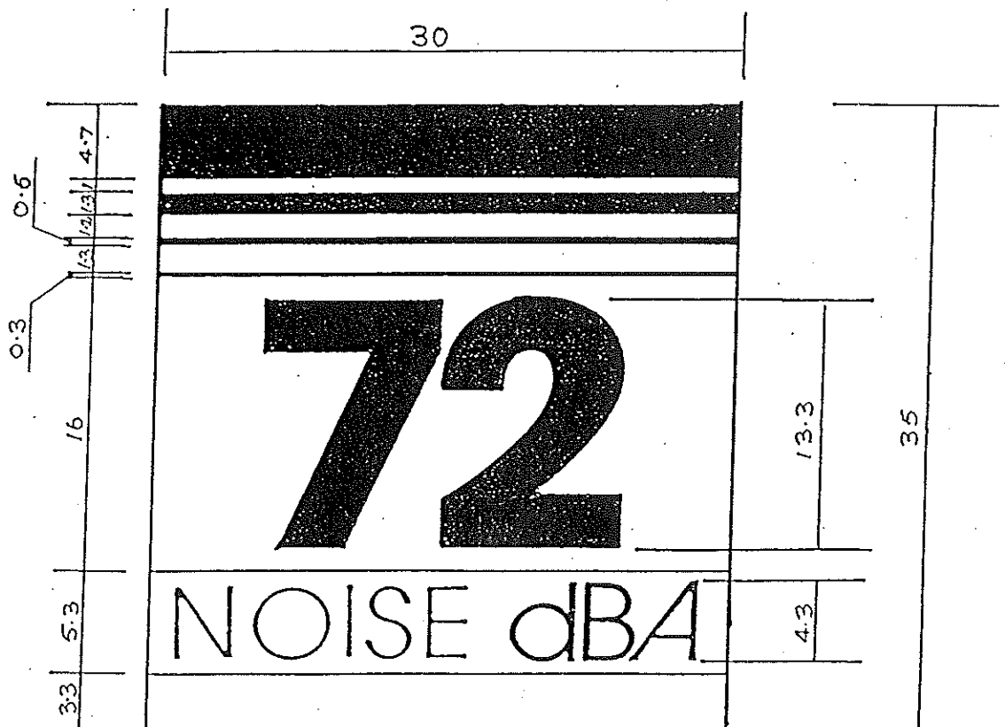
Label dimensions (for Grass Cutting Machines)
