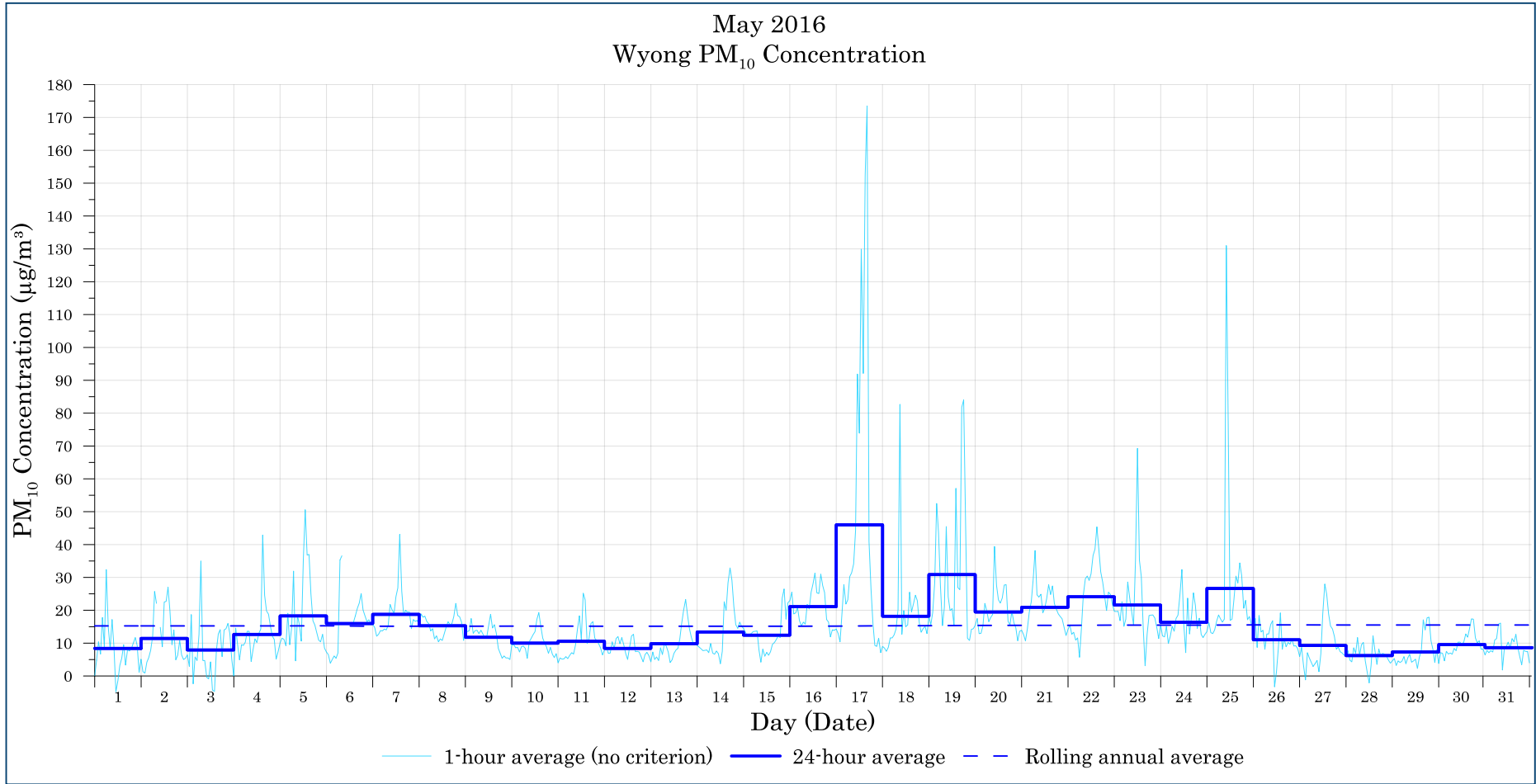
Figure B-2: Wyong PM 10 (1-hour, 24-hour and rolling annual average) concentration – May
