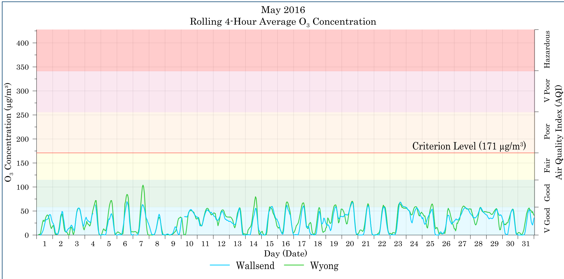
Figure 7-6: Lake Macquarie - Wyong rolling 4-hour average O 3 levels – May 2016
