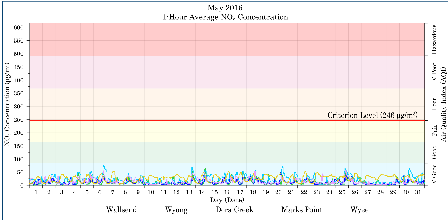
Figure 7-3: Lake Macquarie - Wyong 1-hour average NO 2 levels – May 2016
