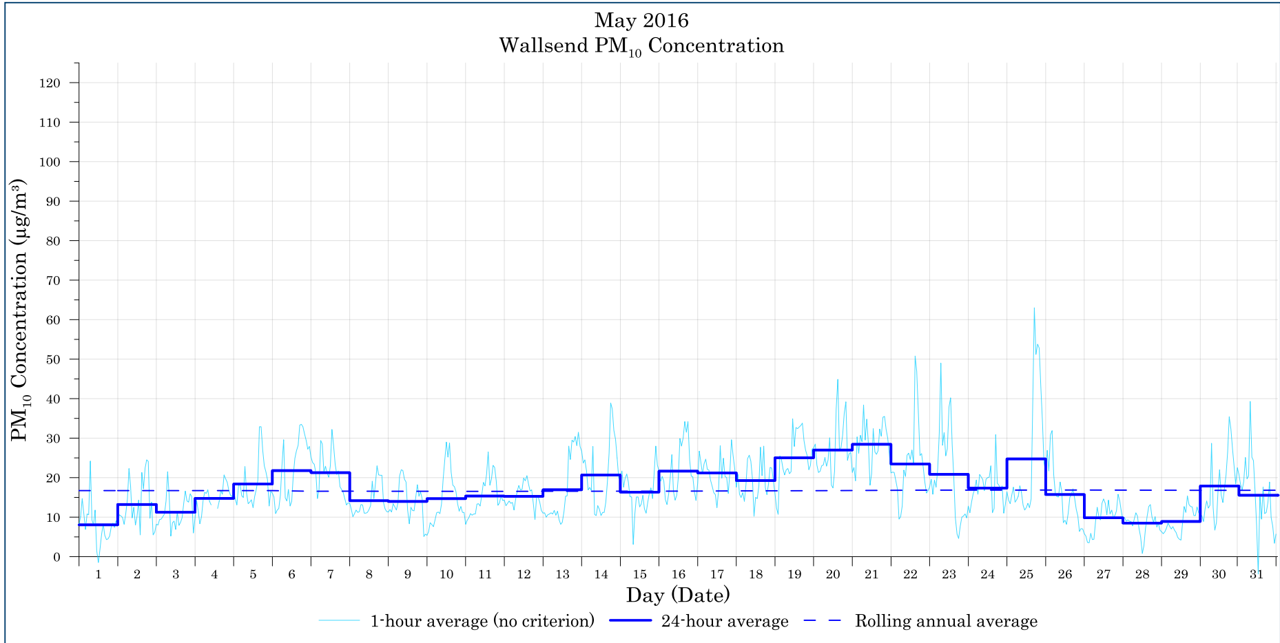
Figure B-1: Wallsend PM 10 (1-hour, 24-hour and rolling annual average) concentration - May
