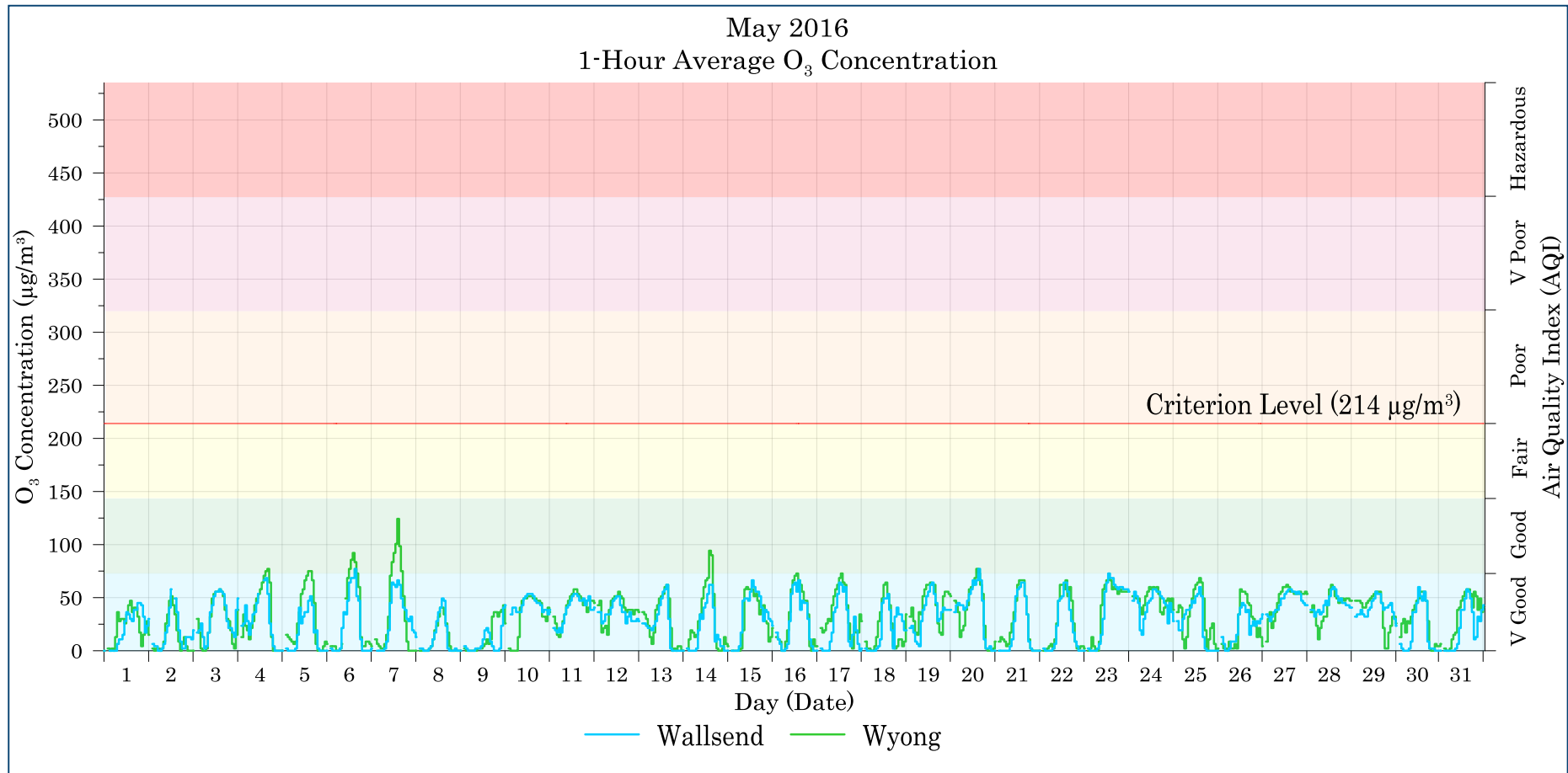
Figure 7-5: Lake Macquarie - Wyong 1-hour average O 3 levels – May 2016
