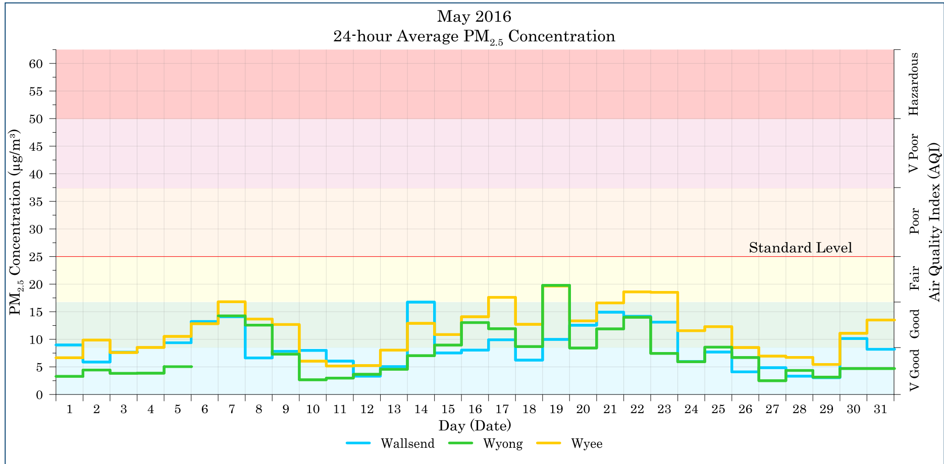
Figure 7-2: Lake Macquarie - Wyong 24-hour average PM 2.5 levels – May 2016
