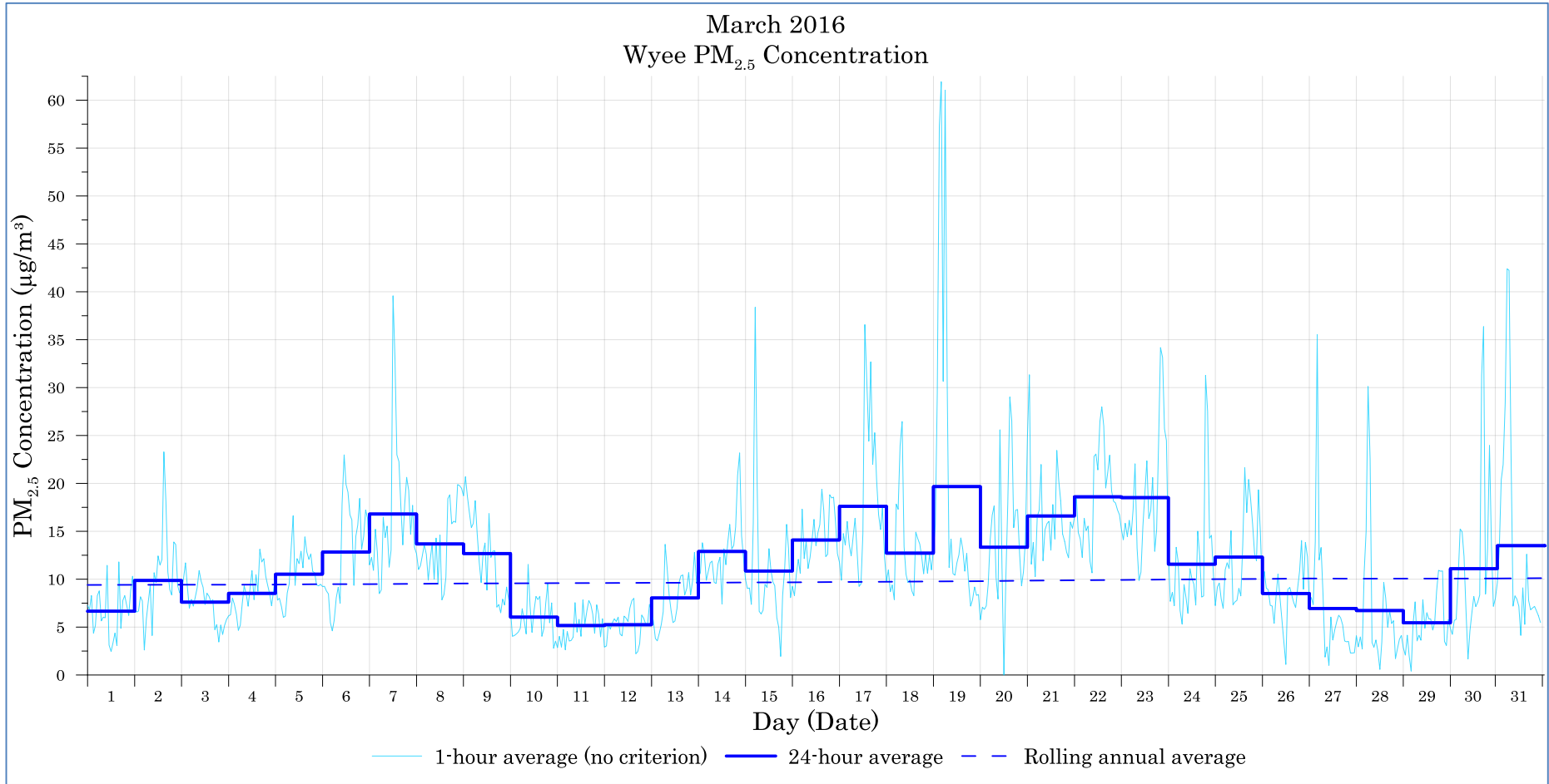
Figure B-5: Wye PM 2.5 (1-hour, 24-hour and rolling annual average) concentration - May
