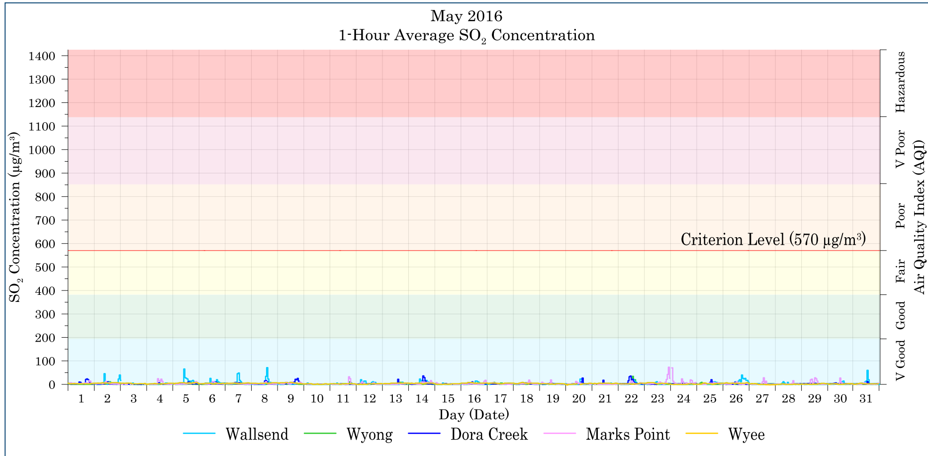
Figure 7-4: Lake Macquarie - Wyong 1-hour average SO 2 levels – May 2016
