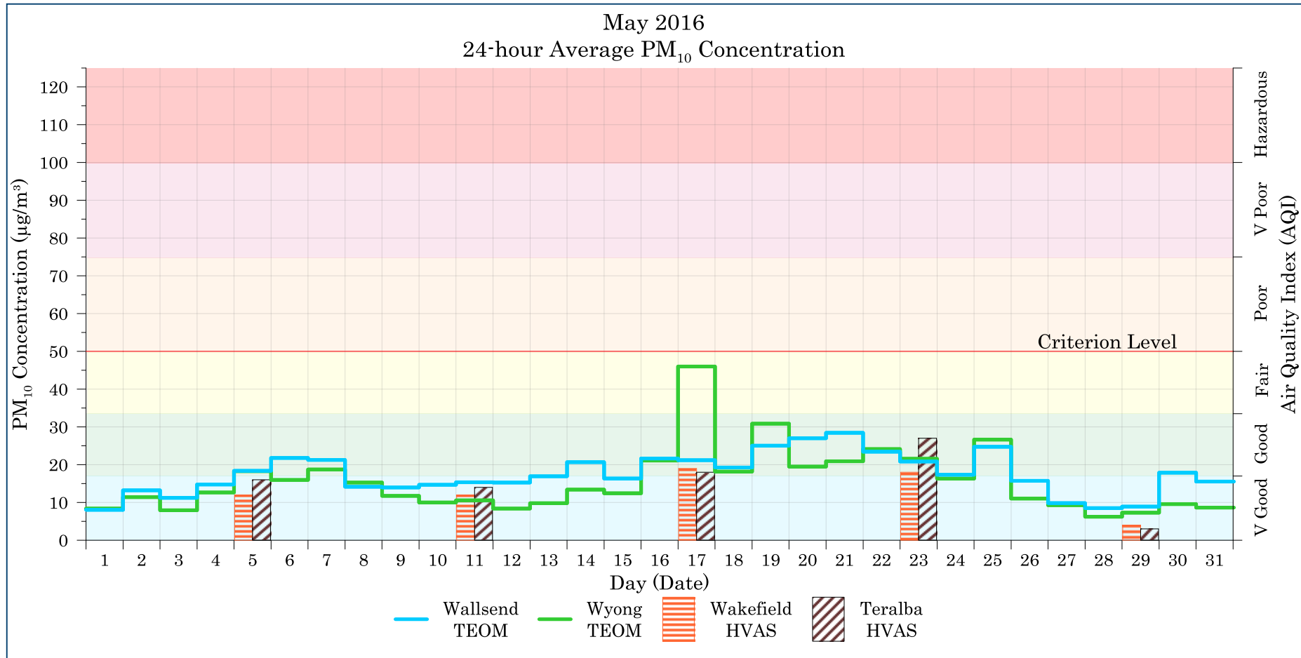
Figure 7-1: Lake Macquarie - Wyong 24-hour average PM 10 levels – May 2016
