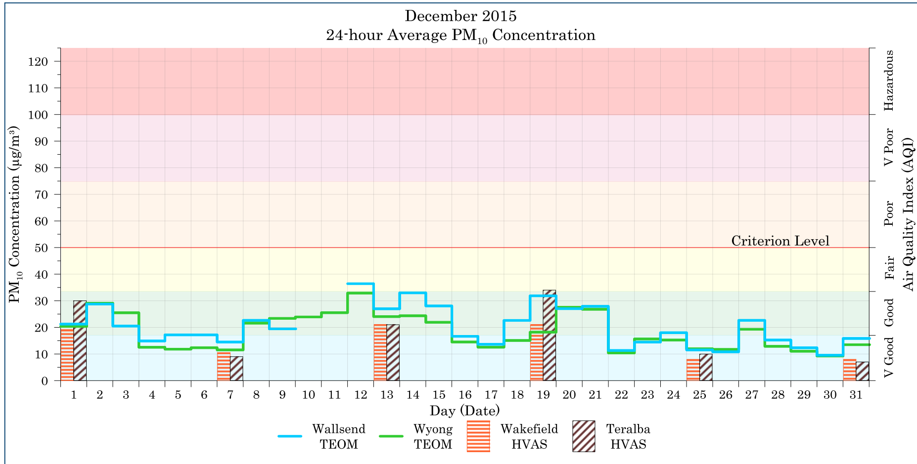
Figure 7-1: Lake Macquarie - Wyong 24-hour average PM 10 levels – December 2015
