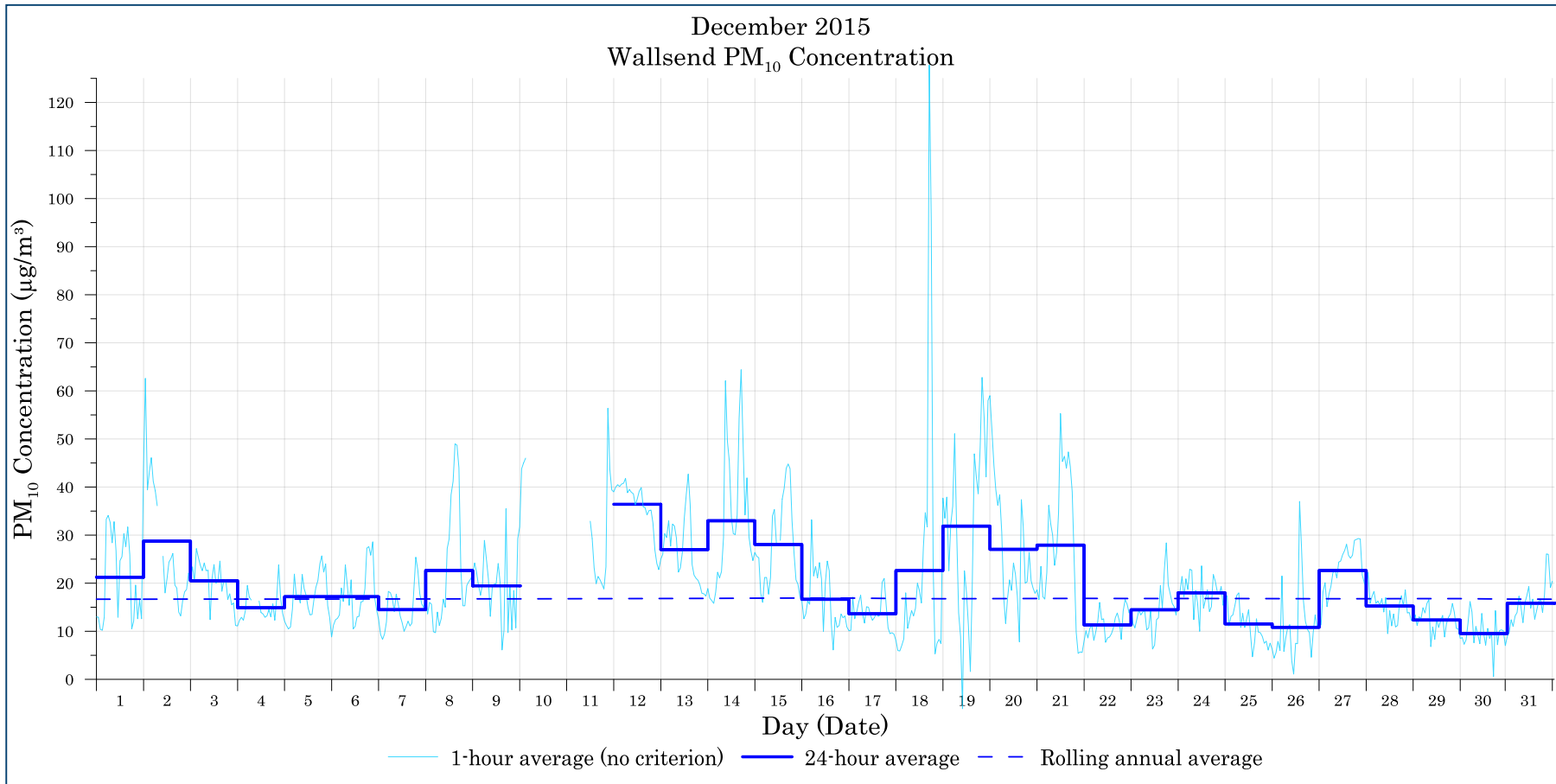
Figure B-1: Wallsend PM 10 (1-hour, 24-hour and rolling annual average) concentration - December
