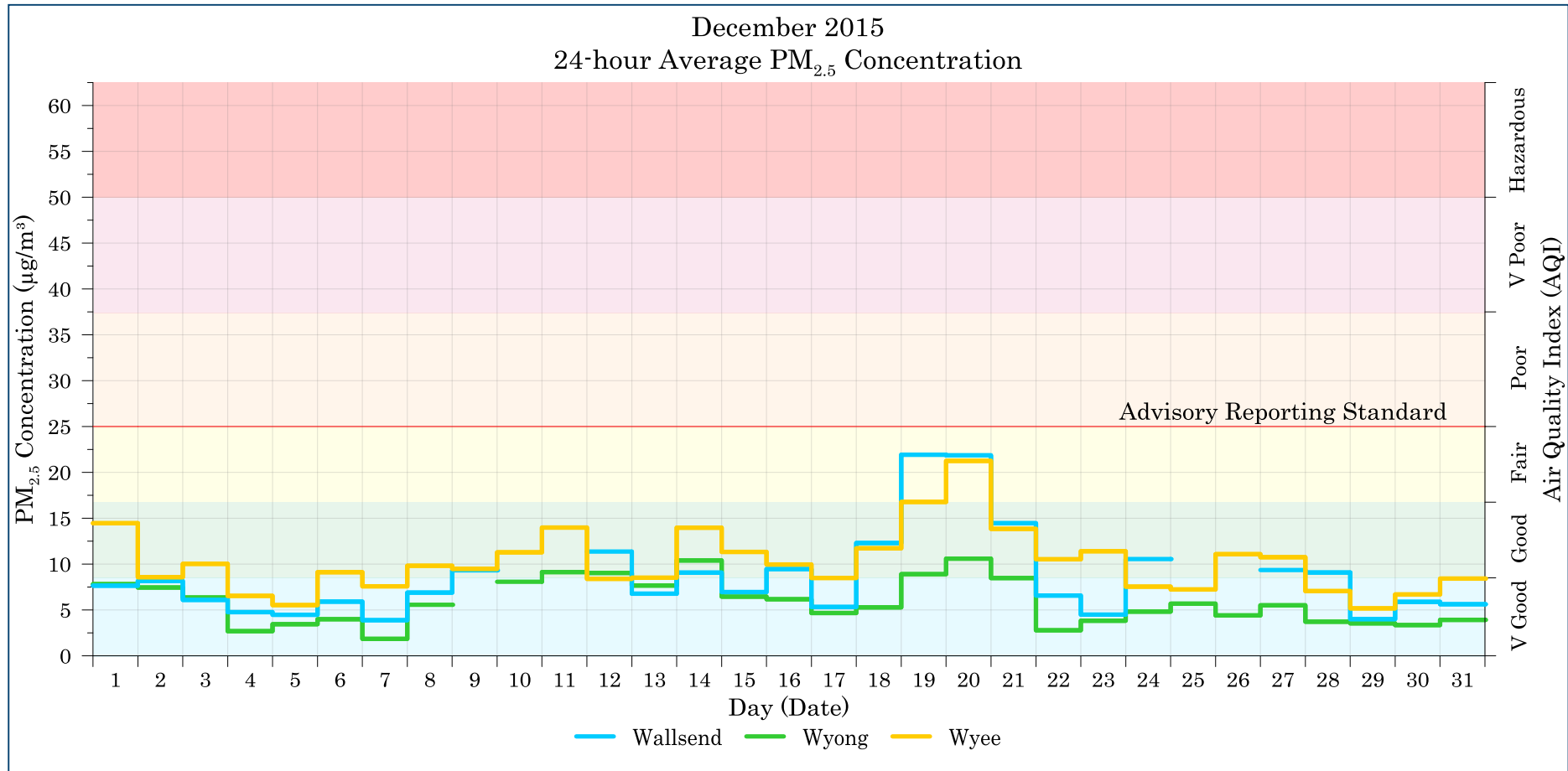
Figure 7-2: Lake Macquarie - Wyong 24-hour average PM 2.5 levels – December 2015
