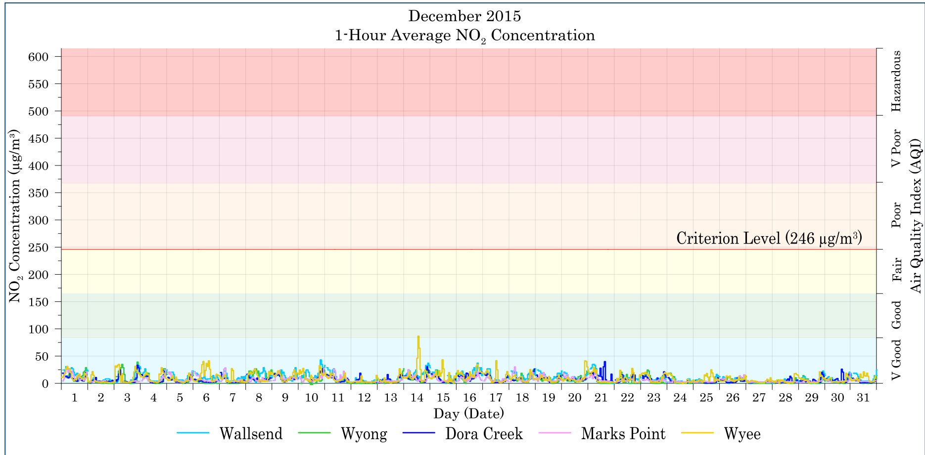
Figure 7-3: Lake Macquarie - Wyong 1-hour average NO 2 levels – December 2015
