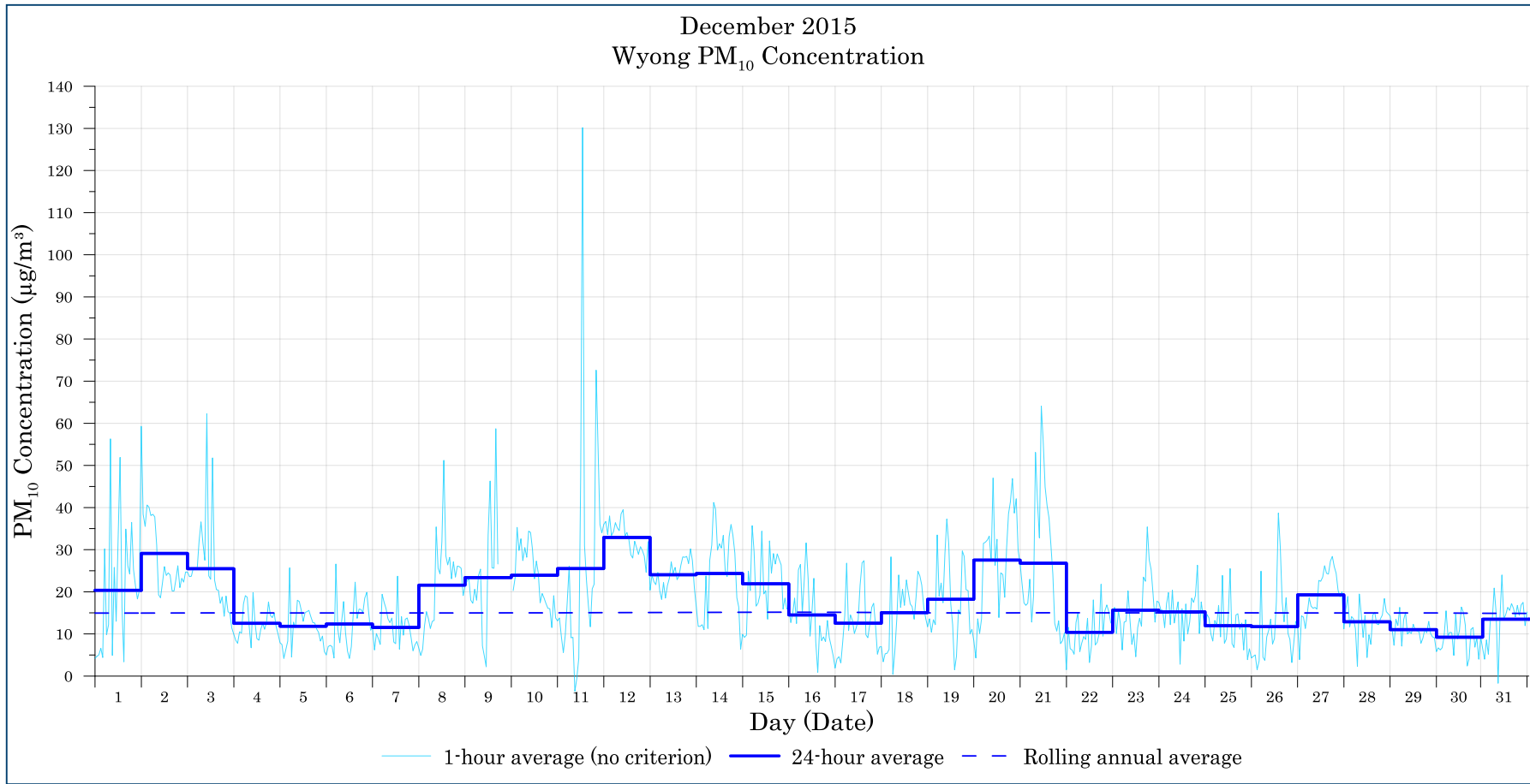
Figure B-2: Wyong PM 10 (1-hour, 24-hour and rolling annual average) concentration – December
