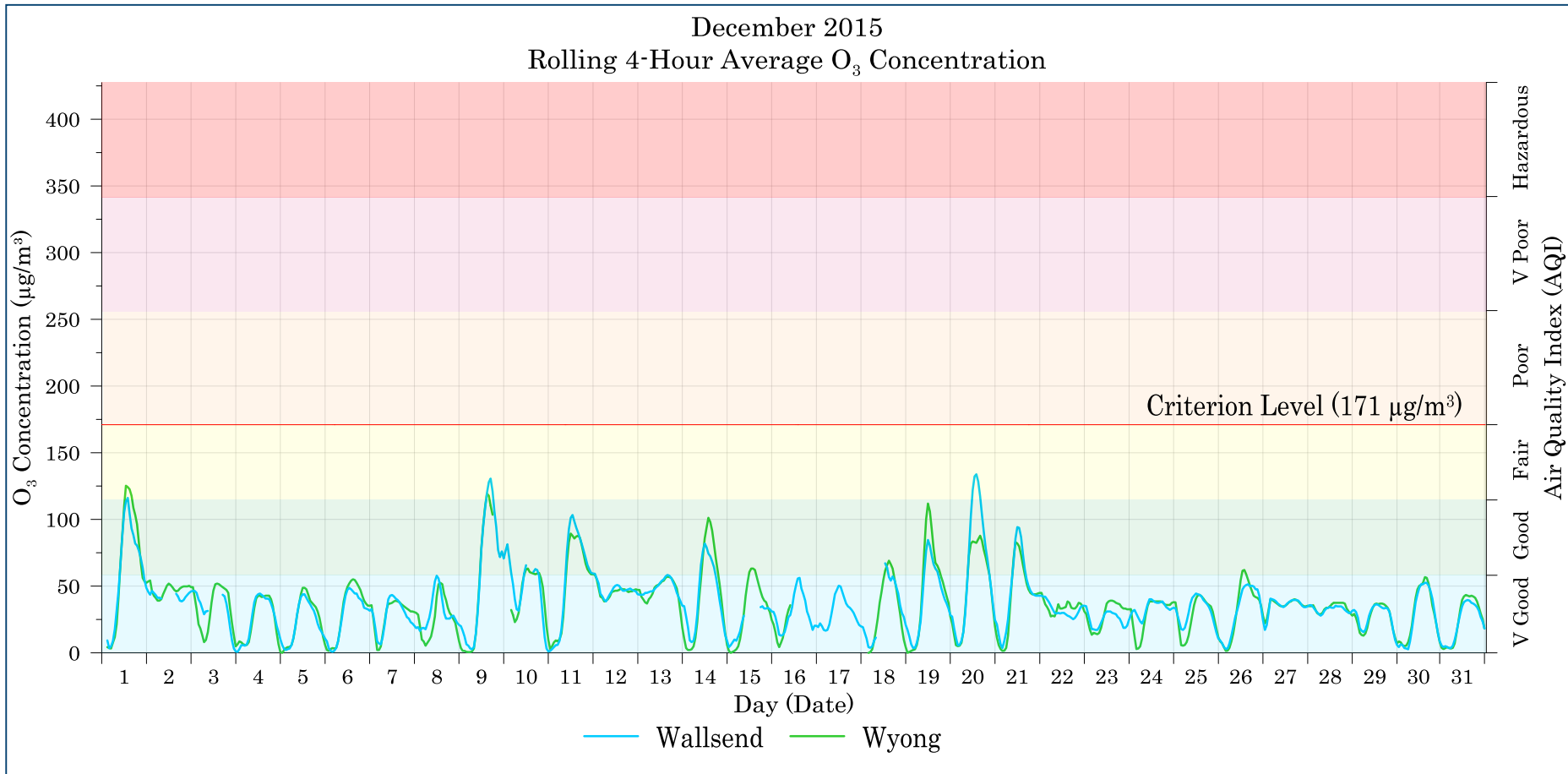
Figure 7-6: Lake Macquarie - Wyong rolling 4-hour average O 3 levels – December 2015
