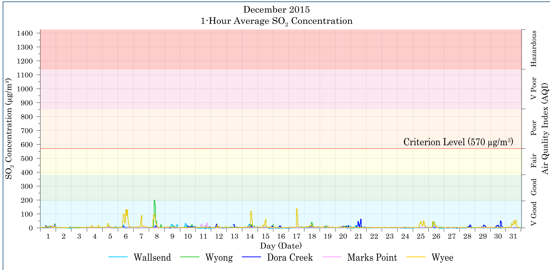
Figure 7-4: Lake Macquarie - Wyong 1-hour average SO 2 levels – December 2015
