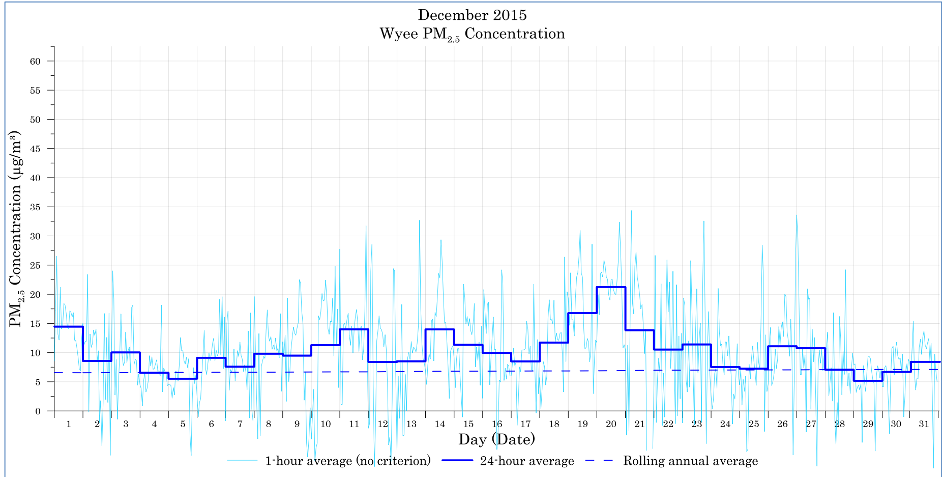
Figure B-5: Wye PM 2.5 (1-hour, 24-hour and rolling annual average) concentration - December
