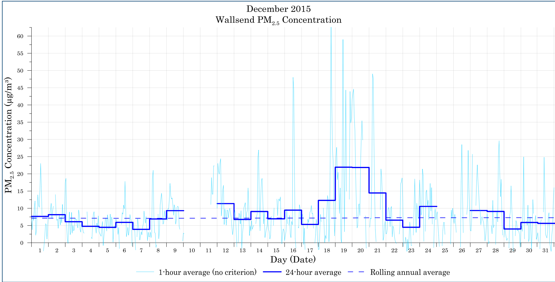
Figure B-3: Wallsend PM 2.5 (1-hour, 24-hour and rolling annual average) concentration – December
