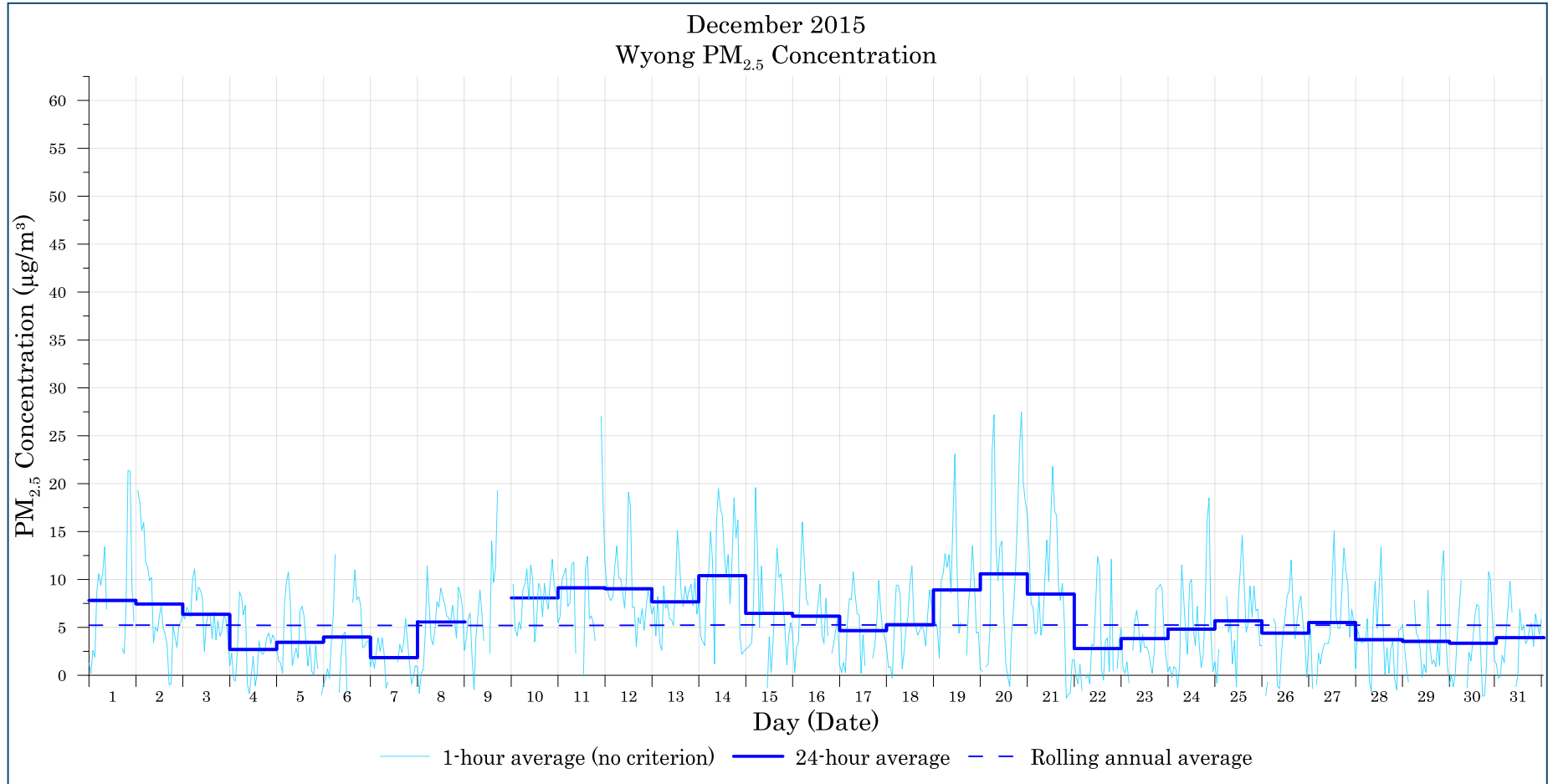
Figure B-4: Wyong PM 2.5 (1-hour, 24-hour and rolling annual average) concentration – December
