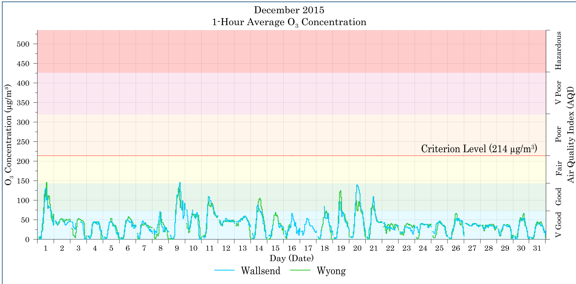
Figure 7-5: Lake Macquarie - Wyong 1-hour average O 3 levels – December 2015
