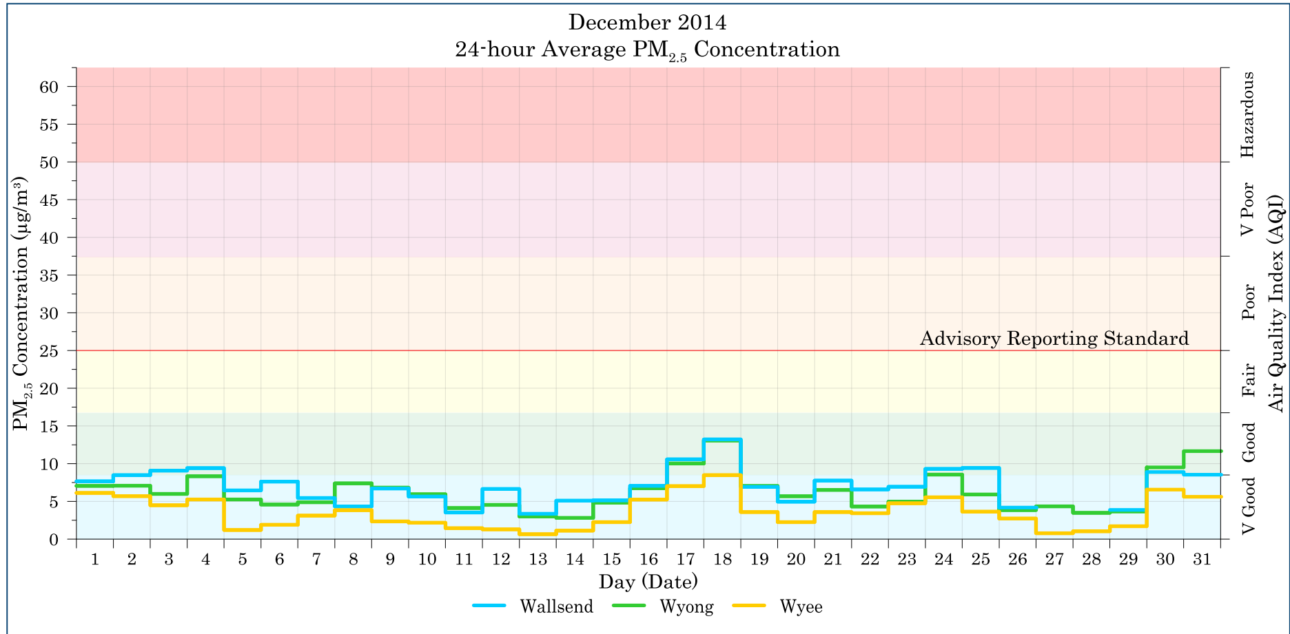
Figure 7-2: Lake Macquarie - Wyong 24-hour average PM 2.5 levels – December 2014
