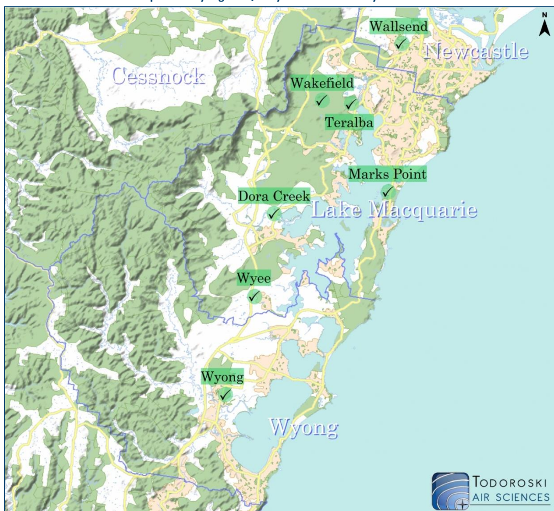
Lake Macquarie – Wyong Air Quality Tabular Summary - December 2014
