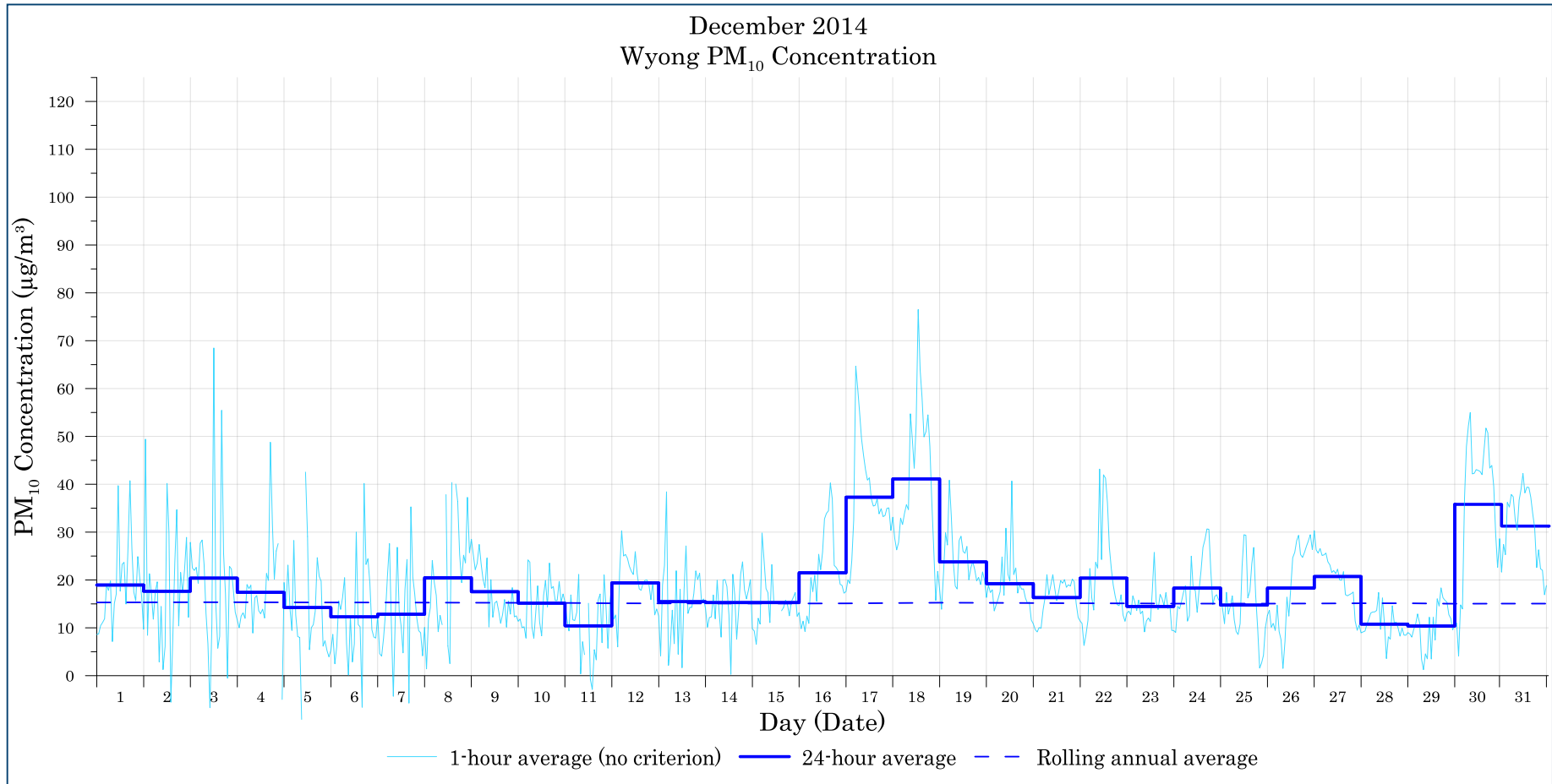
Figure B-2: Wyong PM 10 concentration - December
