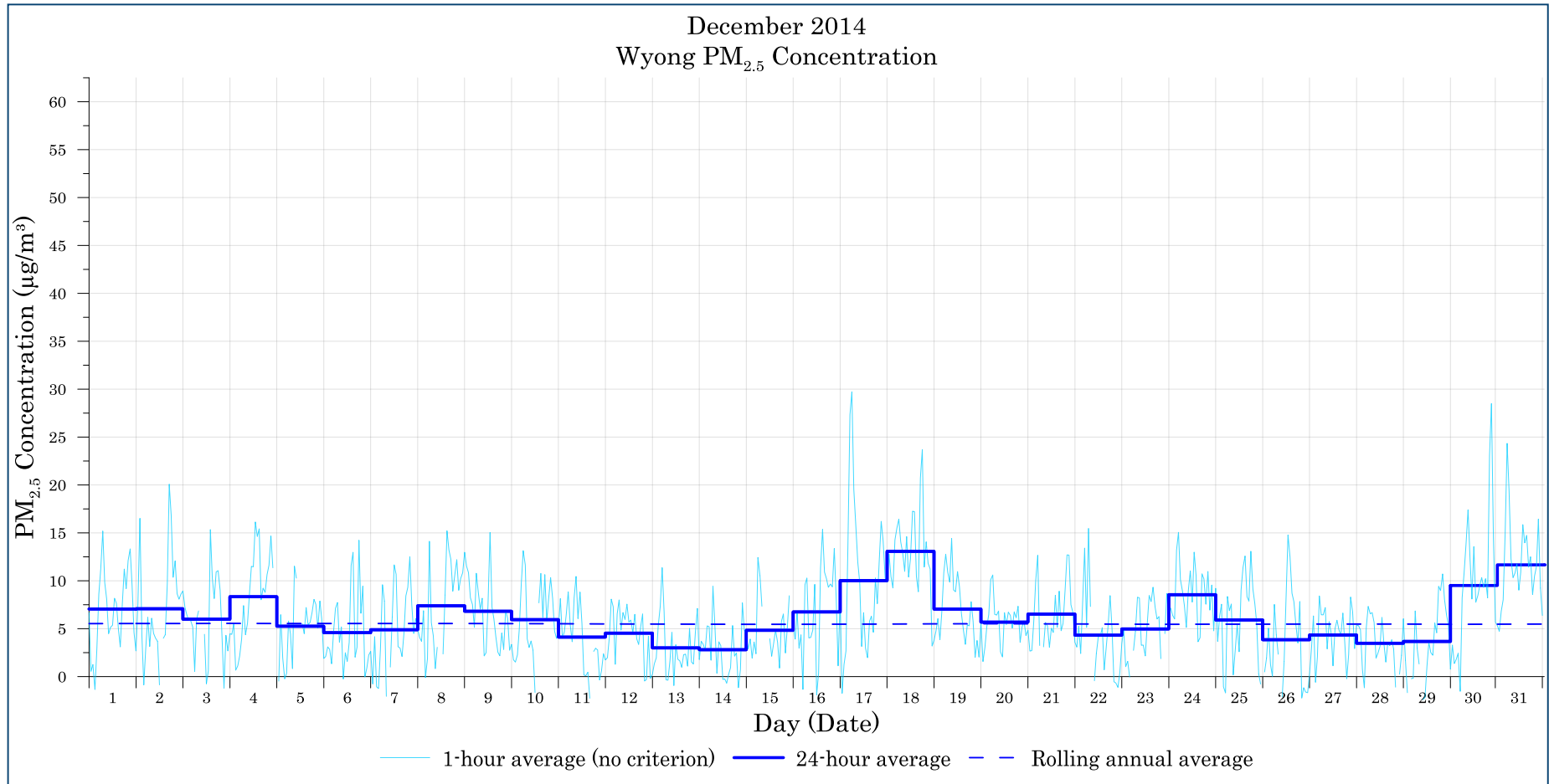
Figure B-4: Wyong PM 2.5 concentration - December
