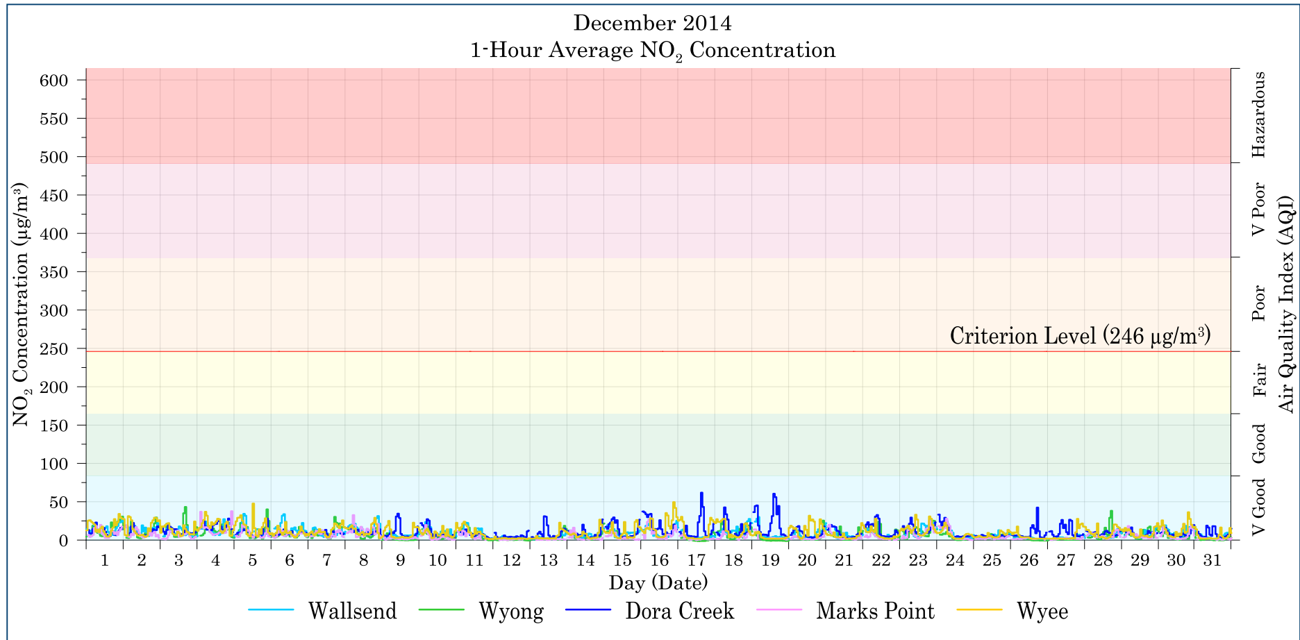
Figure 7-3: Lake Macquarie - Wyong 1-hour average NO 2 levels – December 2014
