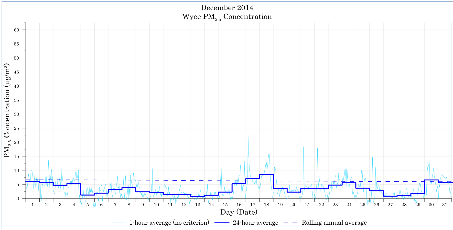
Figure B-5: Wyee PM 2.5 concentration - December
