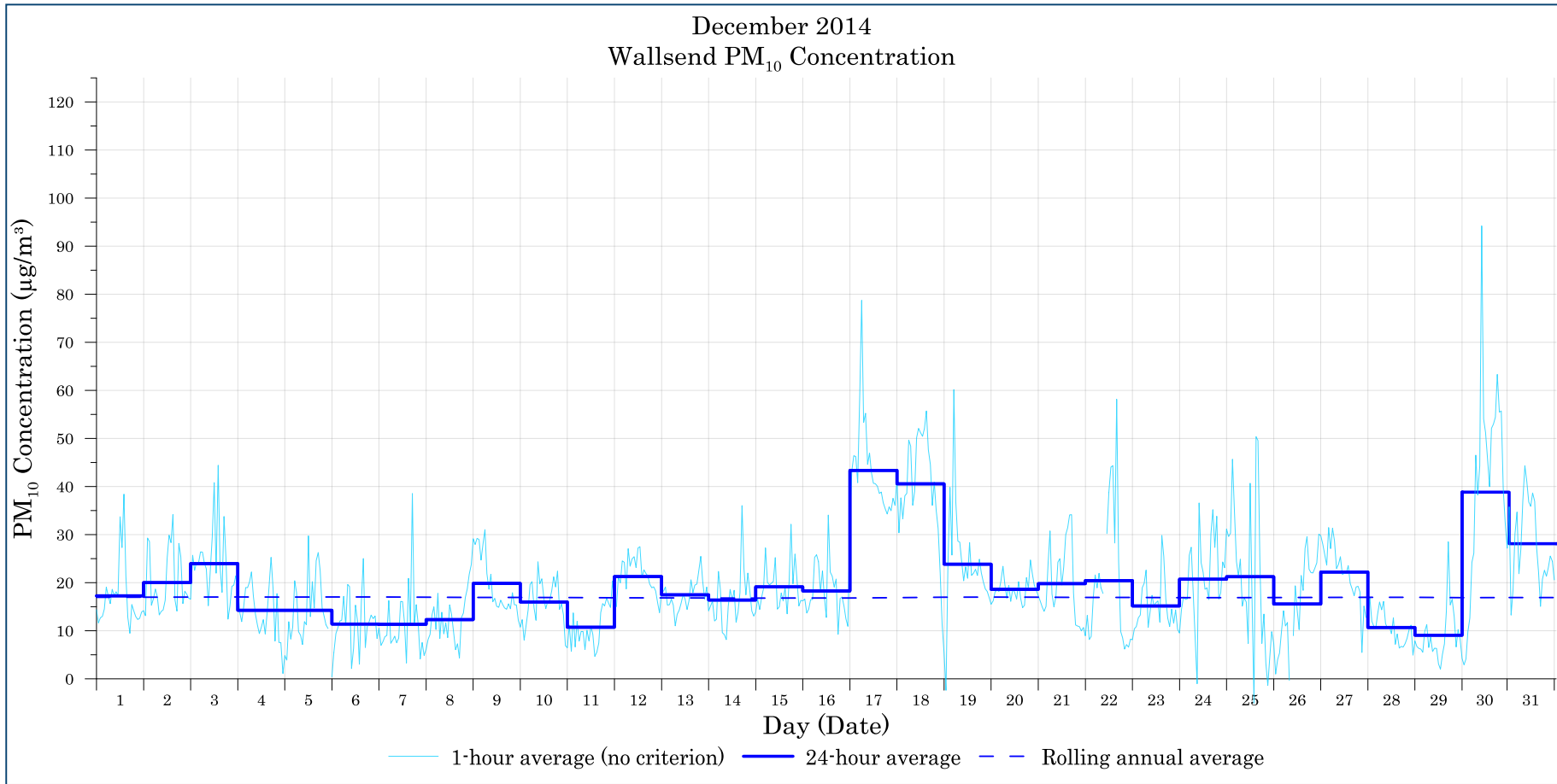
Figure B-1: Wallsend PM 10 concentration - December
