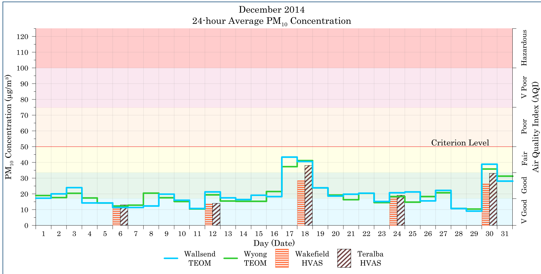
Figure 7-1: Lake Macquarie - Wyong 24-hour average PM 10 levels – December 2014
