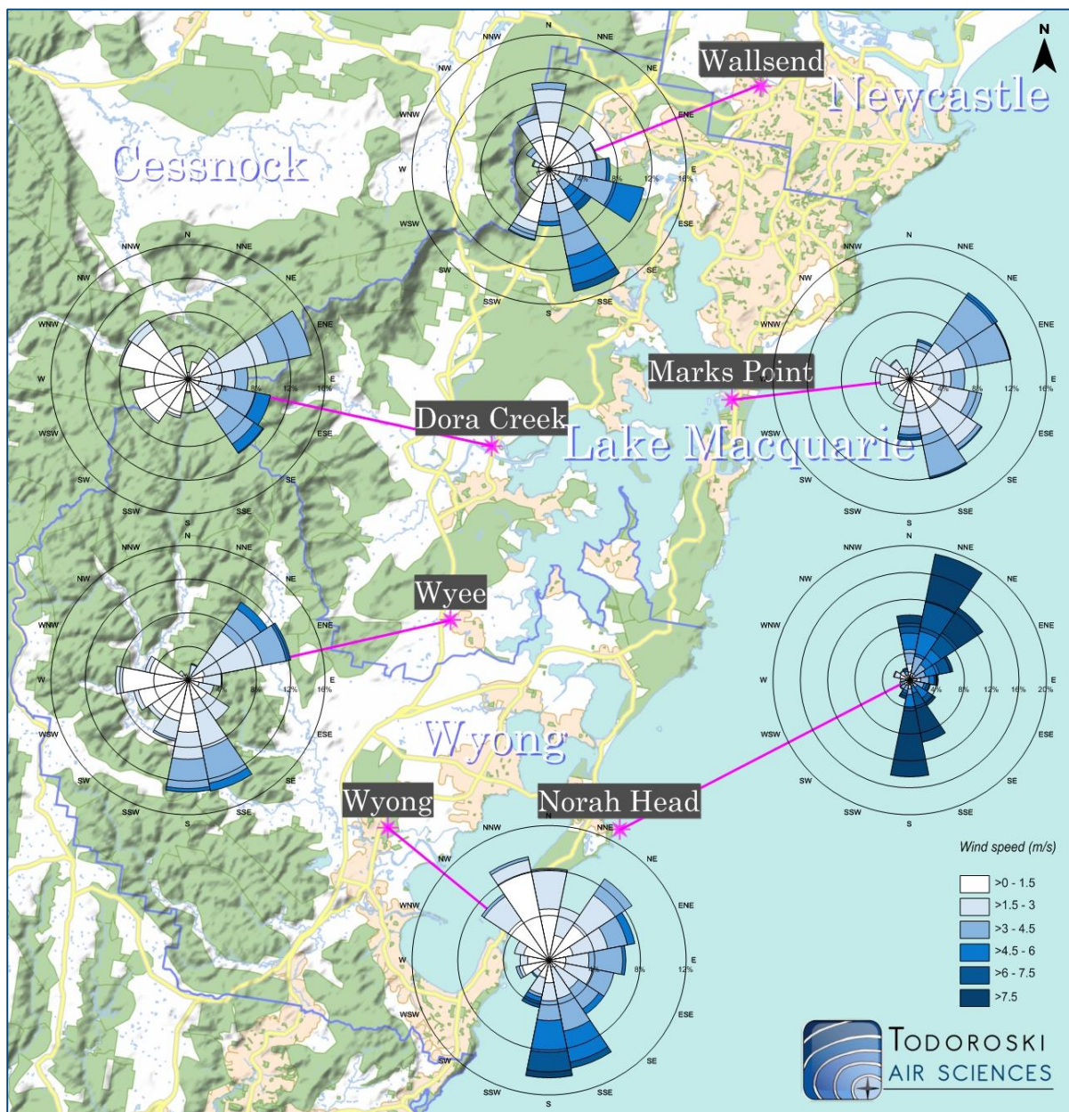
Figure 6-1: December windroses – Wallsend, Dora Creek, Marks Point, Wyee, Norah Head and Wyong
