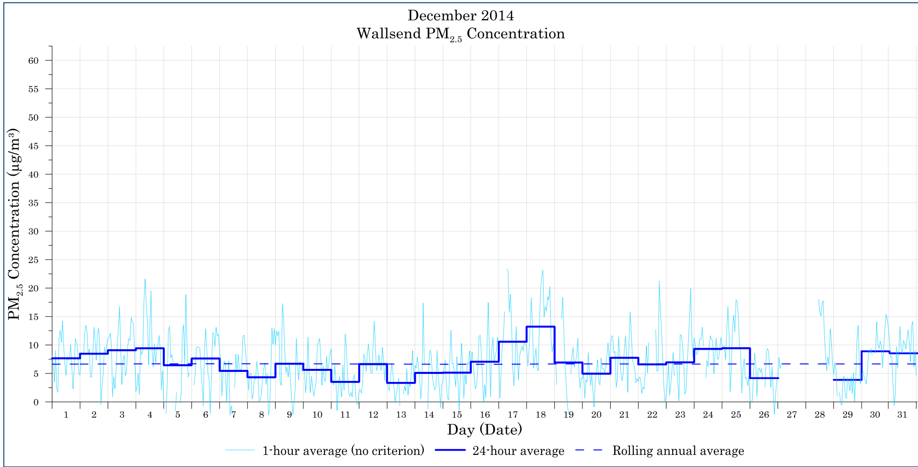
Figure B-3: Wallsend PM 2.5 concentration - December
