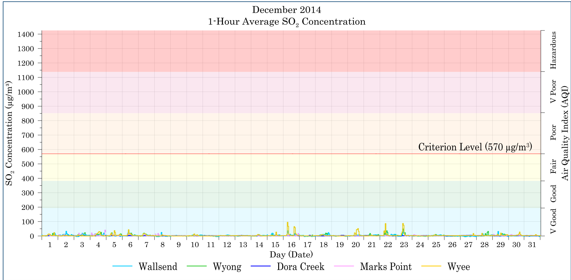
Figure 7-4: Lake Macquarie - Wyong 1-hour average SO 2 levels – December 2014
