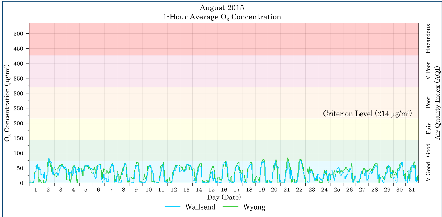
Figure 7-5: Lake Macquarie - Wyong 1-hour average O 3 levels – August 2015
