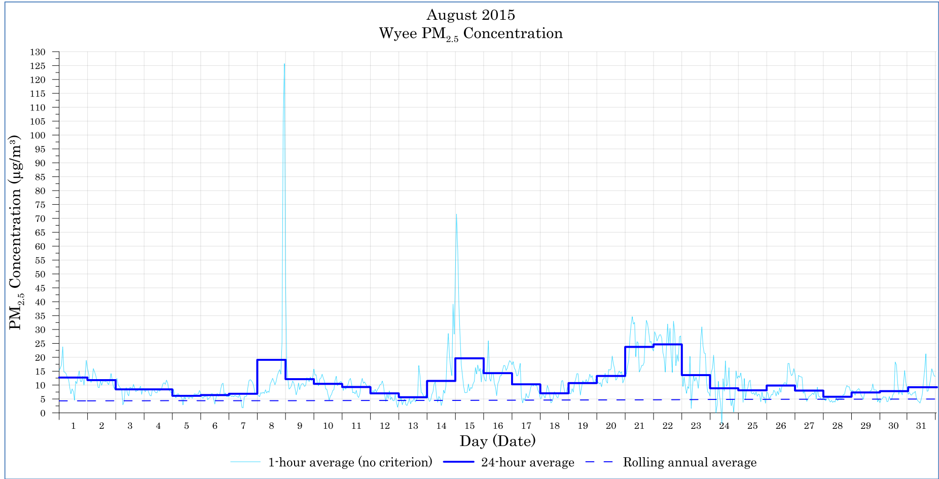
Figure B-5: Wyee PM 2.5 (1-hour, 24-hour and rolling annual average) concentration - August
