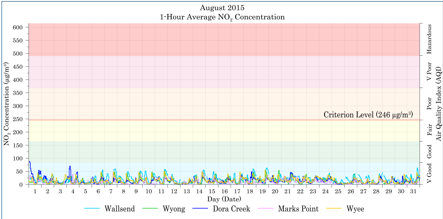
Figure 7-3: Lake Macquarie - Wyong 1-hour average NO 2 levels – August 2015
