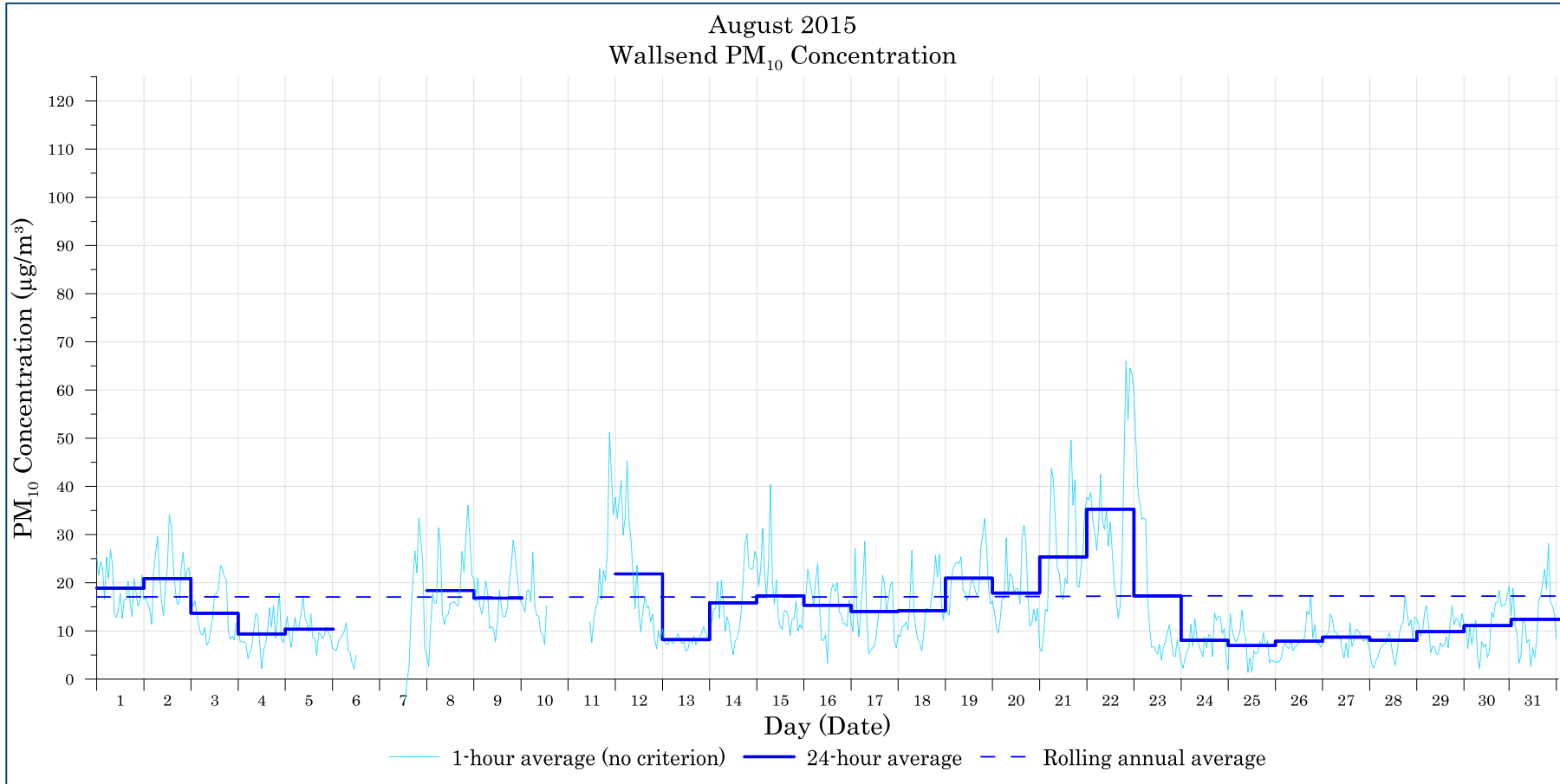
Figure B-1: Wallsend PM 10 (1-hour, 24-hour and rolling annual average) concentration - August
