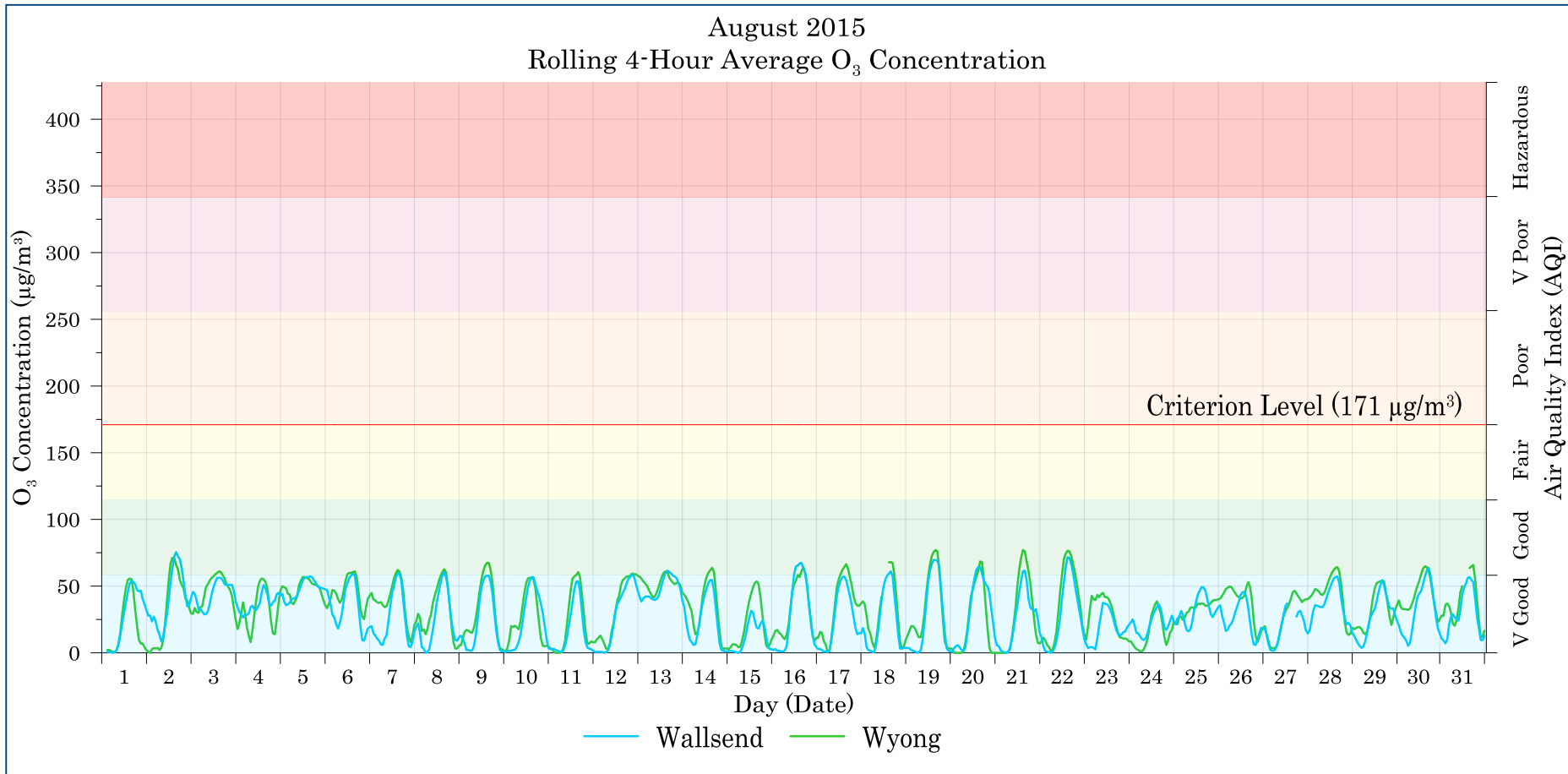
Figure 7-6: Lake Macquarie - Wyong rolling 4-hour average O 3 levels – August 2015
