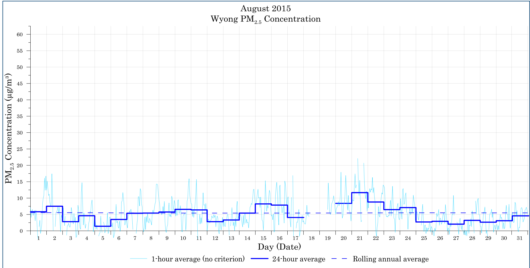
Figure B-4: Wyong PM 2.5 (1-hour, 24-hour and rolling annual average) concentration – August
