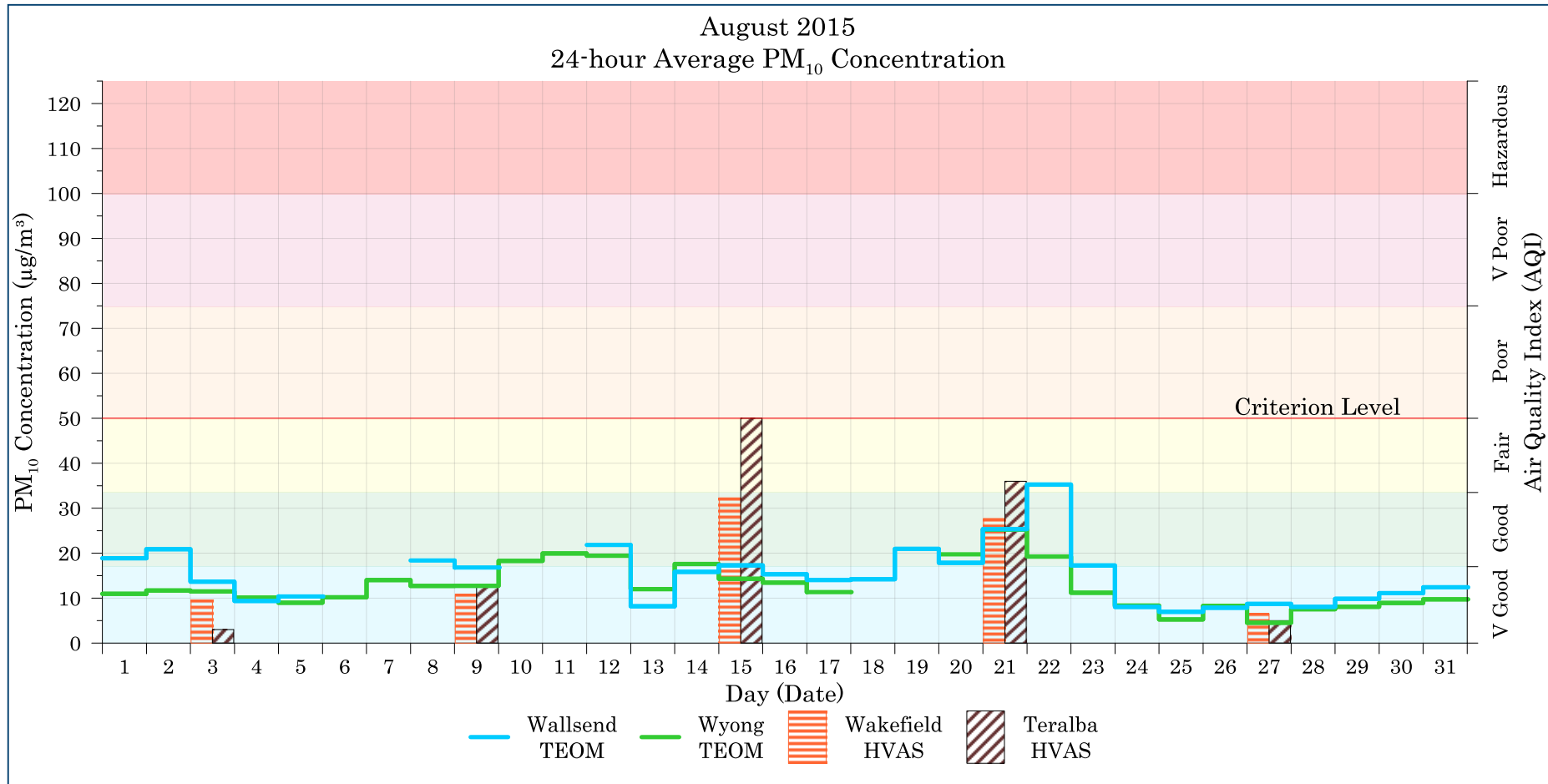
Figure 7-1: Lake Macquarie - Wyong 24-hour average PM 10 levels – August 2015
