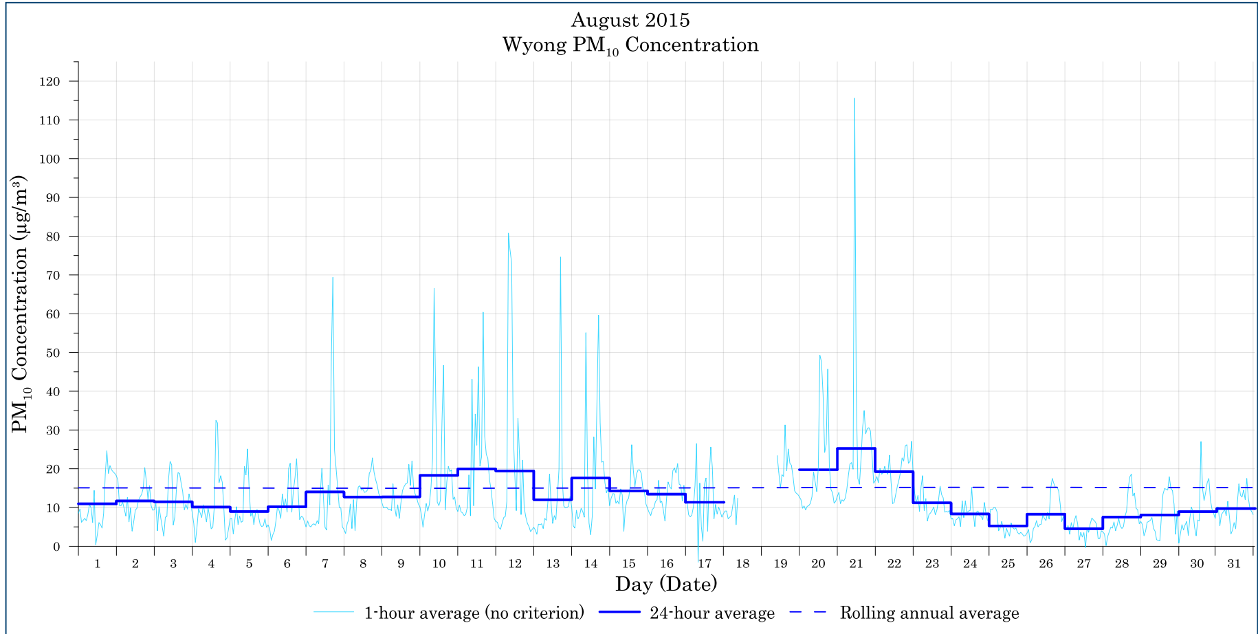
Figure B-2: Wyong PM 10 (1-hour, 24-hour and rolling annual average) concentration – August
