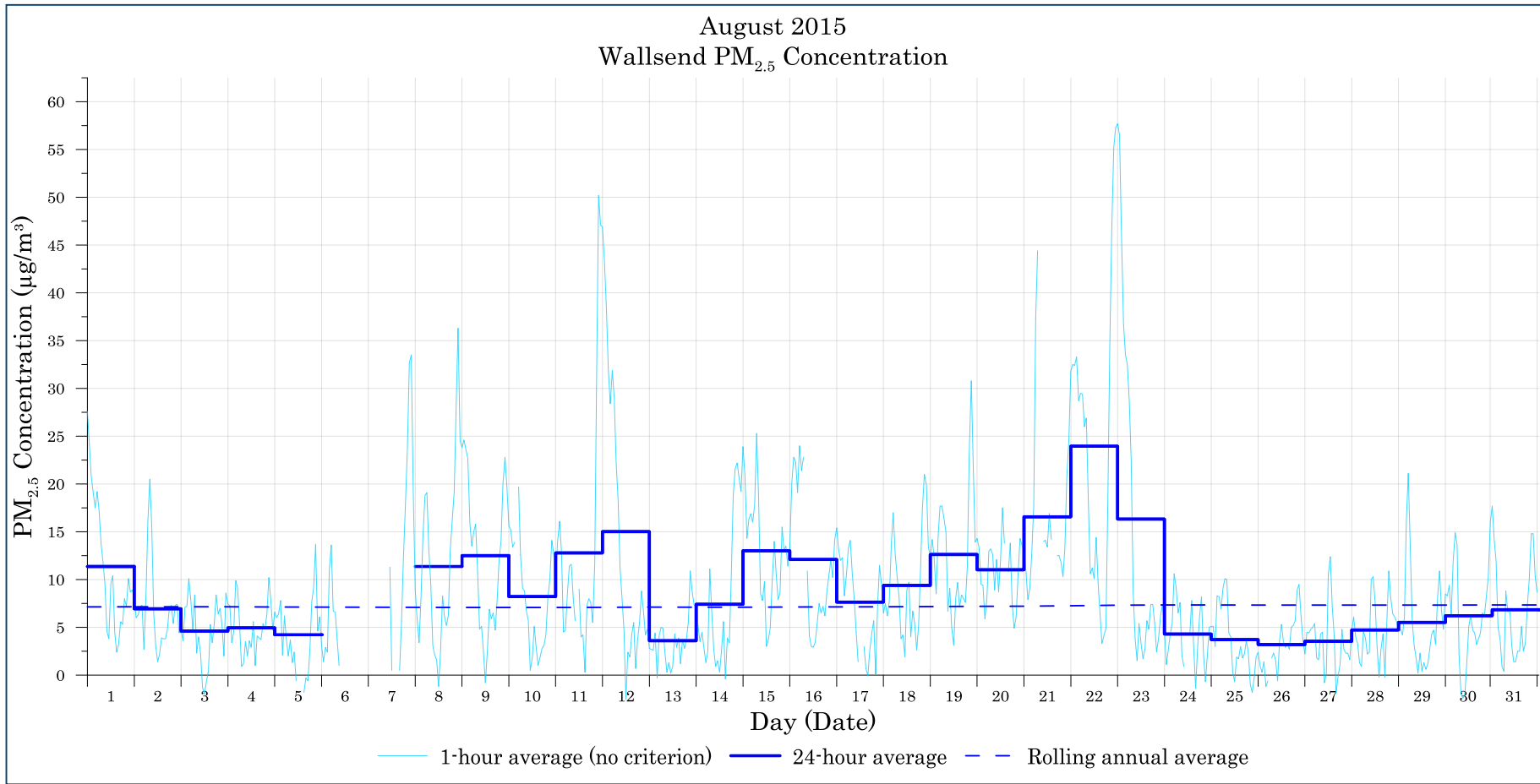
Figure B-3: Wallsend PM 2.5 (1-hour, 24-hour and rolling annual average) concentration – August
